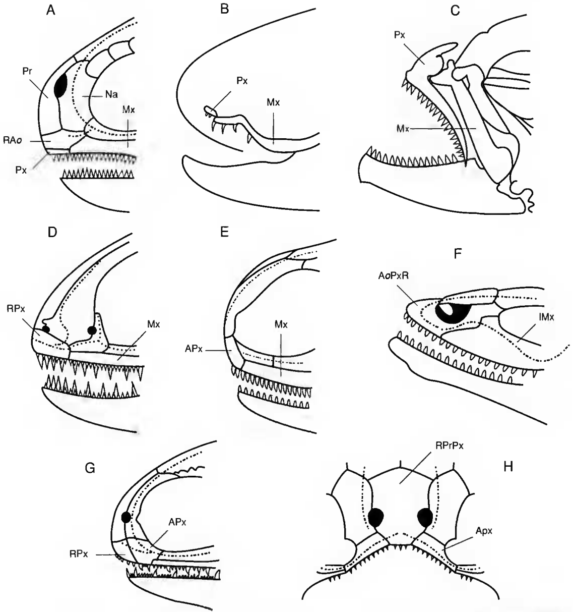
FIG. 1. — Dermal snouts: A-G, left lateral view; H, front view. A, Perleidus piveteaui (after Lehman 1952, fig. 86); B, Polypterus , 9.6 mm larva (after Pehrson 1958, fig. 8); C, Pomatomus saltatrix (after Gregory 1933, fig. 177); D, Birgeria groenlandica (after Nielsen 1949, fig. 69); E, Moythomasia nilida (after Jessen 1968, fig. 1); F, Polypterus adult (after Daget 1958, fig. 1791); G, Watsonichthys pectinatus (after Gardiner 1963, fig. 1); H, Howqualepis rostridens (after Long 1988, fig. 14B). APx, antorbito-premaxillary; AoPxR, antorbito-premaxillo-rostral; IMx, infraorbital-maxillary; Mx, maxillary; Na, nasal; Px, premaxillary; Pr, postrostral; RAo, rostral-antorbital; RPx, rostral-premaxillary; RPrPx, rostral-postrostral-premaxillary.
